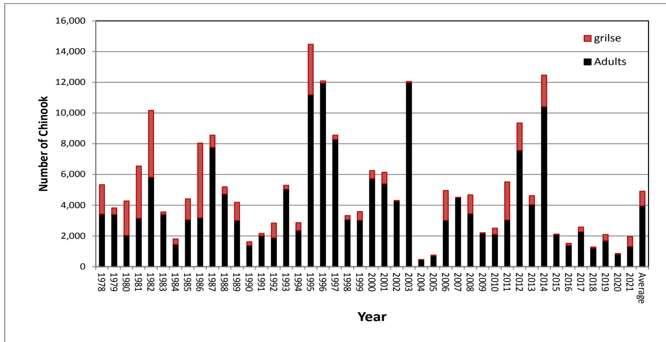
Figure 13. Estimated escapement of Chinook Salmon returning to the Scott River from 1978 to 2021.
