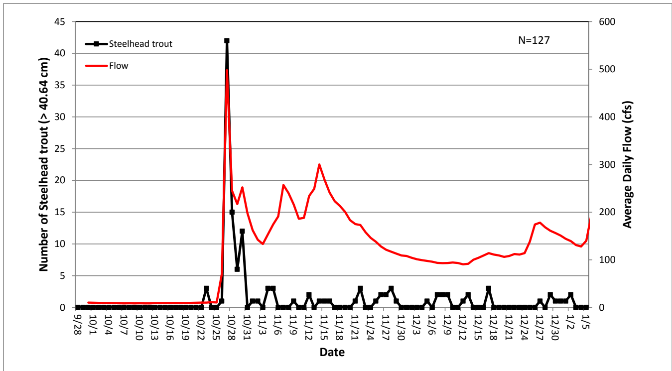
Figure 12. Run timing of steelhead trout (>40.64 cm) observed passing through the Scott River Fish Counting Facility during the 2021 season (N=127), and average daily flows observed at USGS Gauge No. 11519500.
