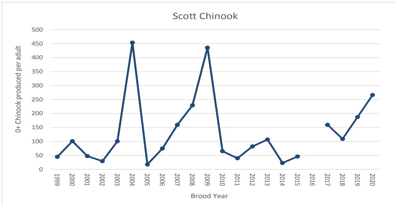
Figure 16. Number of 0+ Chinook Salmon produced per adult spawner in the Scott River by brood year, for Brood Years 1999-2015, 2017-2020.
