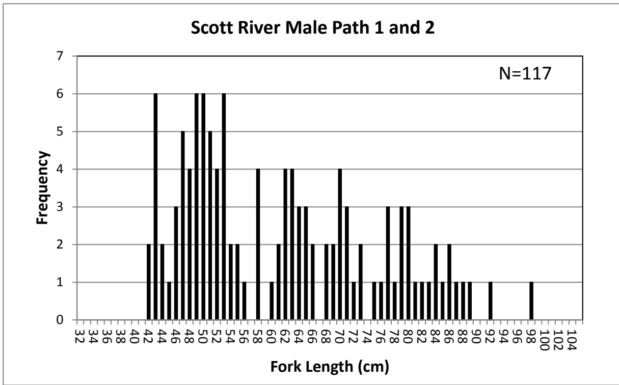
Figure 7. Length Frequency distribution of Path 1 and Path 2 male Chinook Salmon observed during spawning ground surveys in the Scott River, 2021 (N=117).
