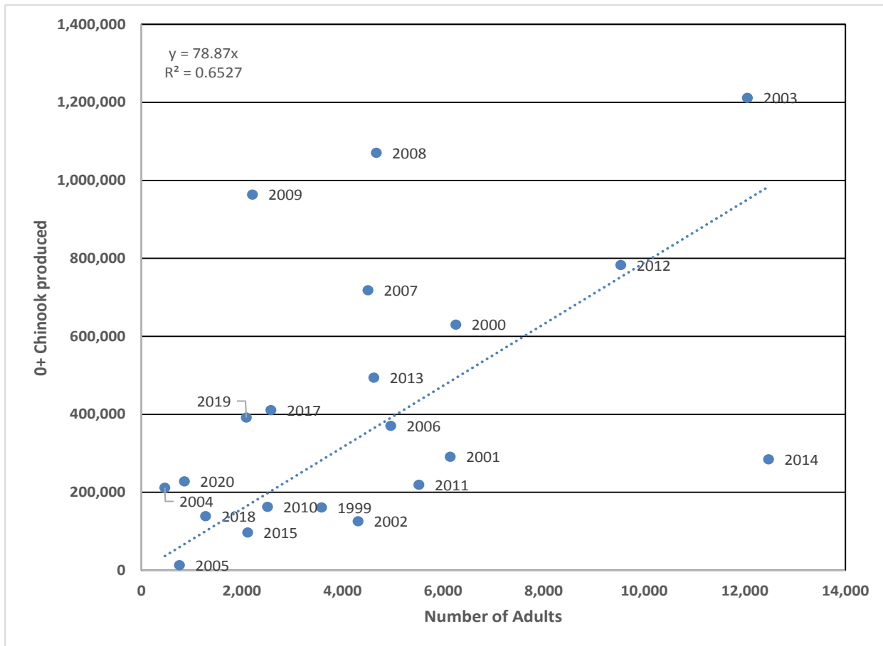
Figure 17. Number of returning adults and corresponding number of 0+ Chinook Salmon produced by year in the Scott River by brood year, for Brood Years 1999-2015, 2017-2020.
