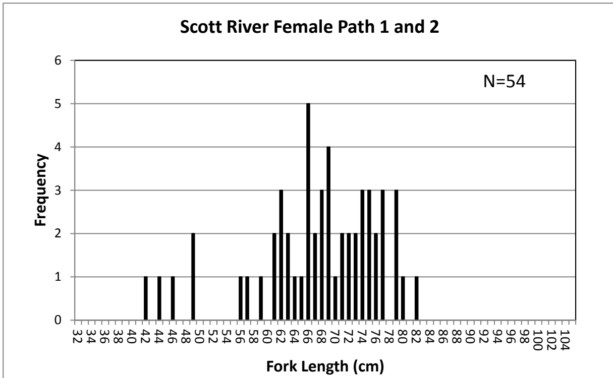
Figure 8. Length frequency distribution of Path 1 and Path 2 female Chinook Salmon observed during spawning ground surveys in the Scott River, 2021 (N=54)
