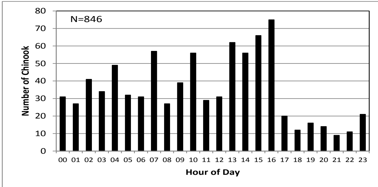
Figure 6. Summary of daily run timing of Chinook Salmon observed at the Scott River Fish Counting Facility during 2021 (N=846).
