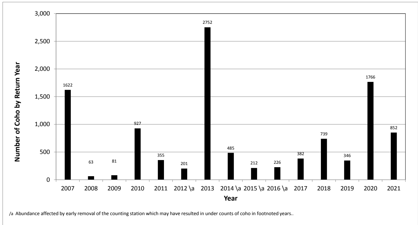
Figure 18. Estimated escapement by return year of adult and grilse Coho Salmon (age 2 and age 3) returning to the Scott River from 2007 to 2021.
