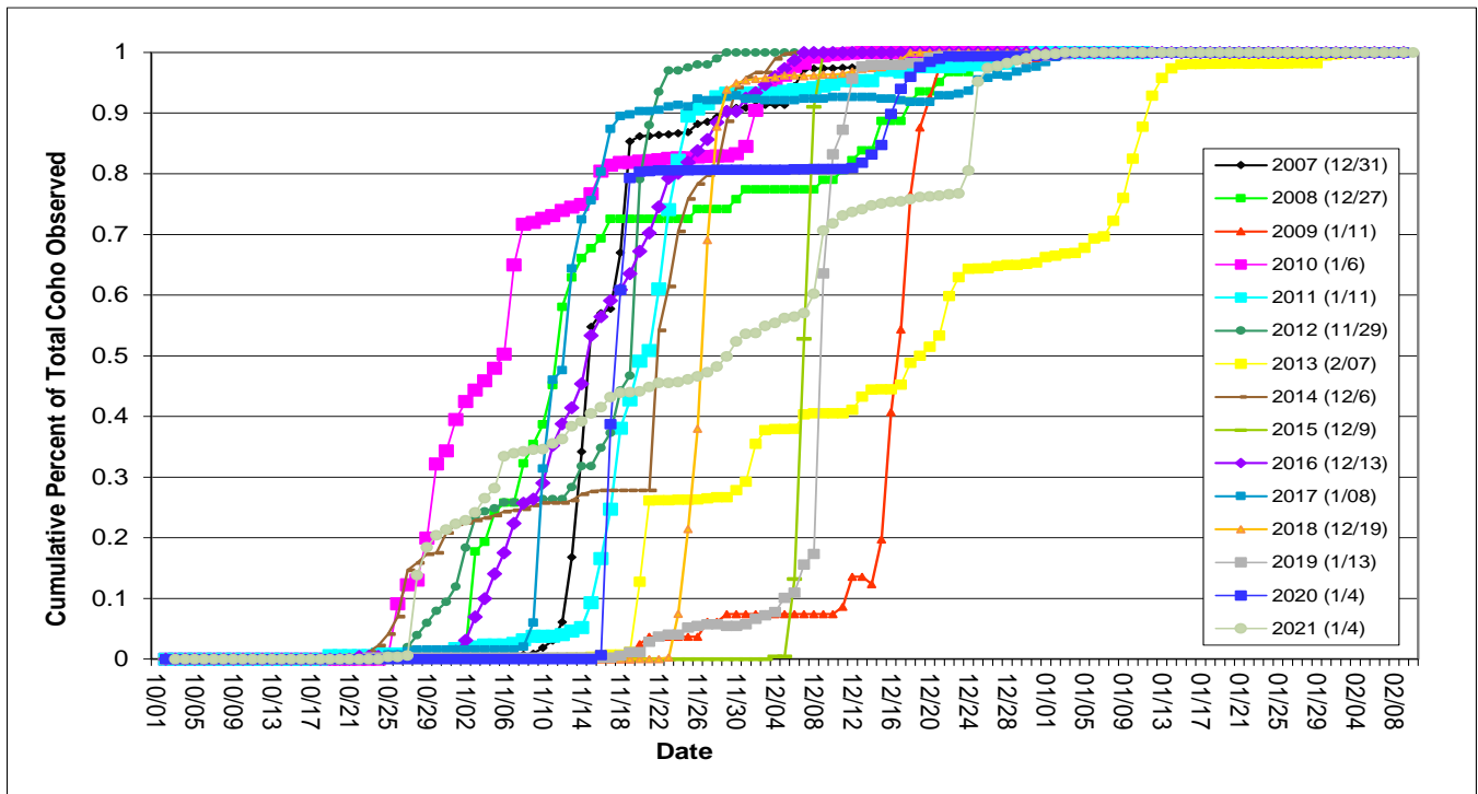
Figure 20. Cumulative percent of total Coho Salmon observations by day at the Scott River Fish Counting Facility annually from 2007-2021. The date in parenthesis indicates the last date the fish counting facility was operated for each year.
