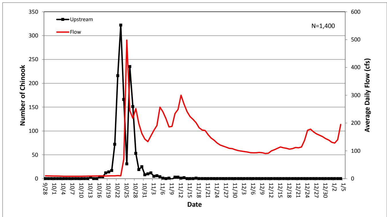
Figure 5. Run timing of Chinook Salmon through the Scott River Fish Counting Facility during the 2021 season (N=1,400), and average daily flows observed at USGS Gauge No. 11519500.
