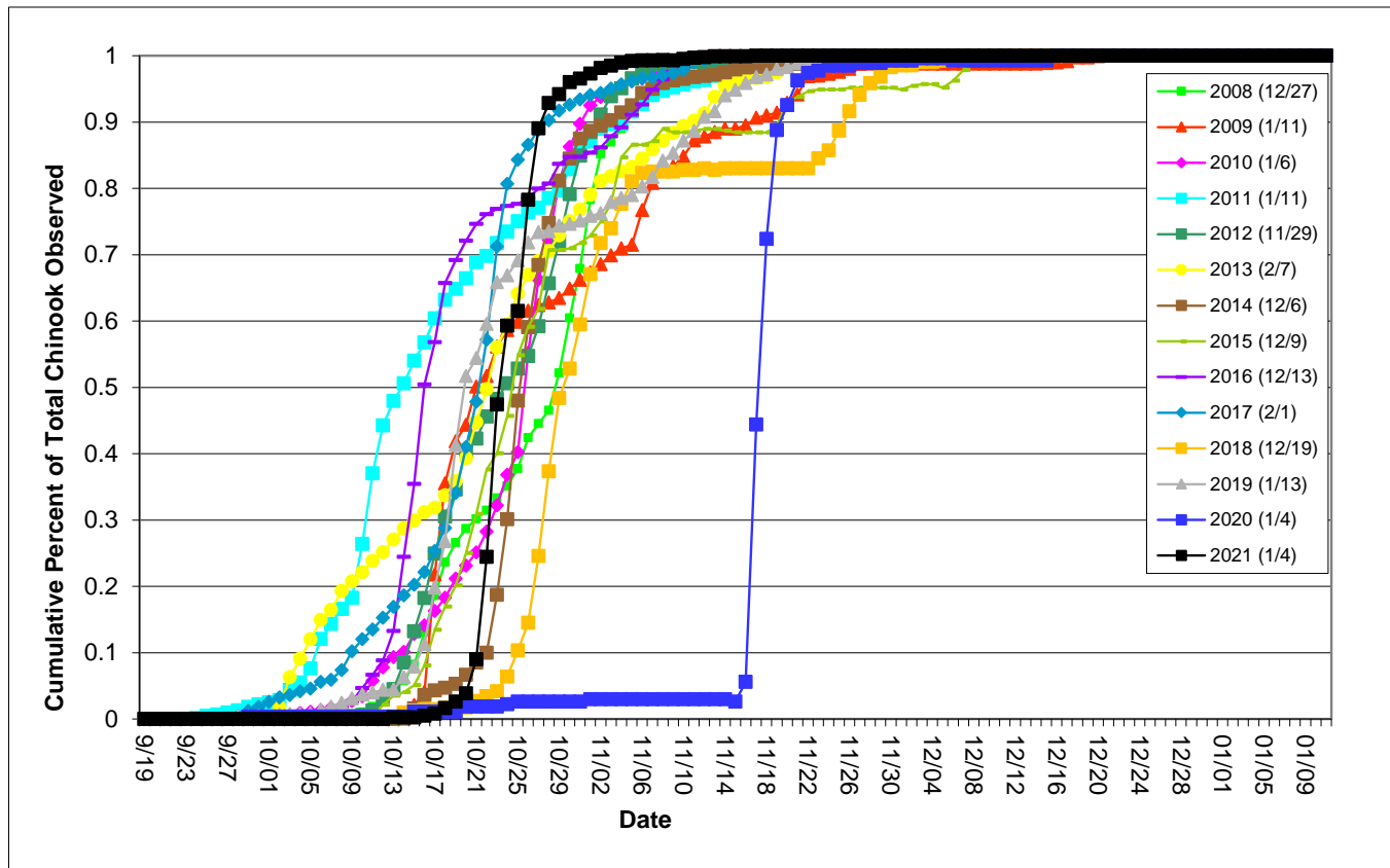
Figure 14. Cumulative percent of total Chinook Salmon observations by day at the Scott River Fish Counting Facility annually from 2008-2021. The date in parenthesis indicates the last date the fish counting facility was operated for each year.
