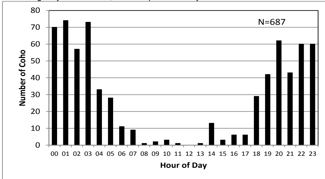
Figure 10. Diel migration patterns of Coho Salmon observed moving through the Scott River Fish Counting Facility in 2021 (N=687).
