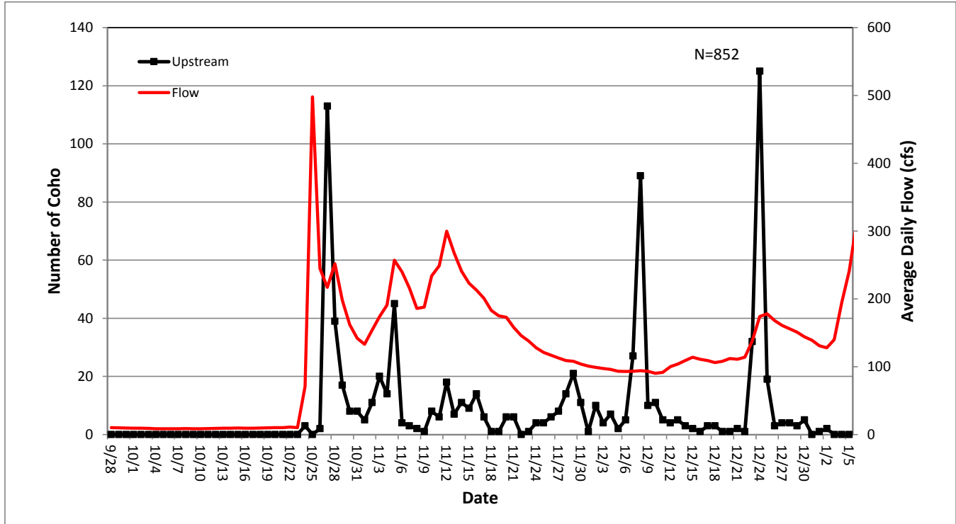
Figure 9. Run timing of Coho Salmon observed passing through the Scott River Fish Counting Facility during the 2021 season (N=852), and average daily flows observed at USGS Gauge No. 11519500.
