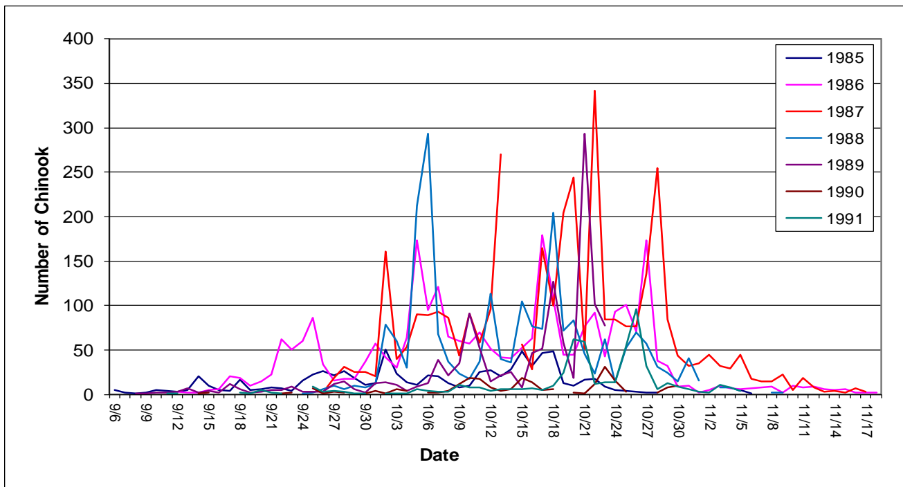
Figure 2. Chinook Salmon observed in the lower Scott River (river mile 1.6) during trapping efforts from 1985-1991.
