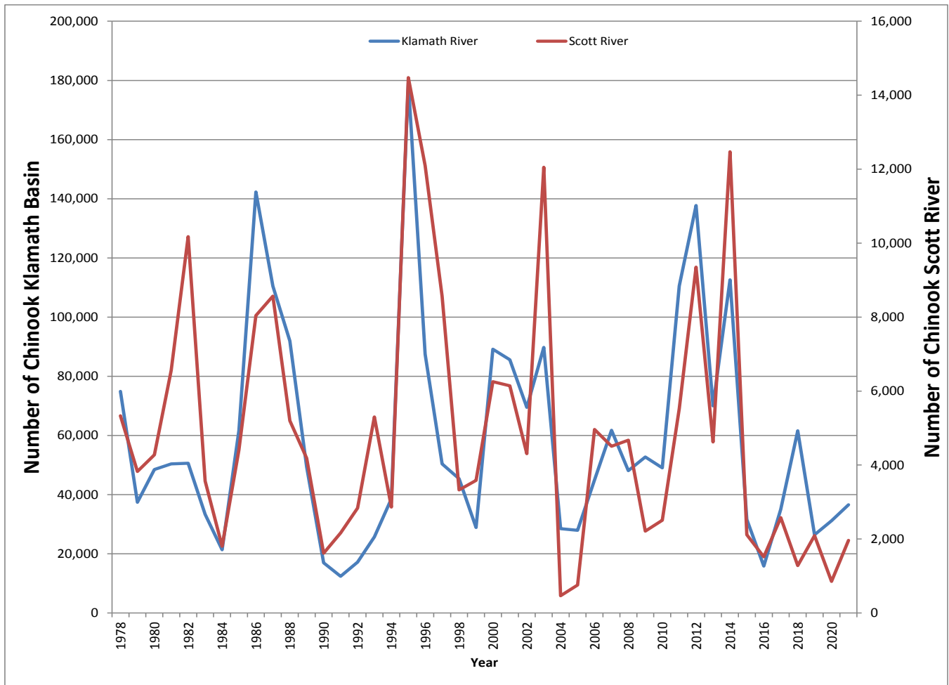
Figure 15. Chinook Salmon Klamath Basin natural spawner escapement (primary y-axis) and the Scott River natural spawner escapement (secondary y-axis) from 1978 through 2021.
