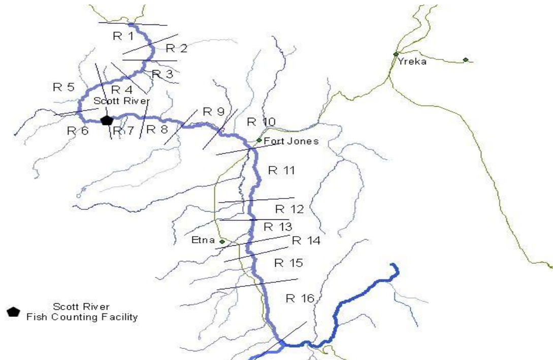
Figure 4. Location of the Scott River Fish Counting Facility and spawning ground survey reaches on the Scott River used during the 2021 field season.
