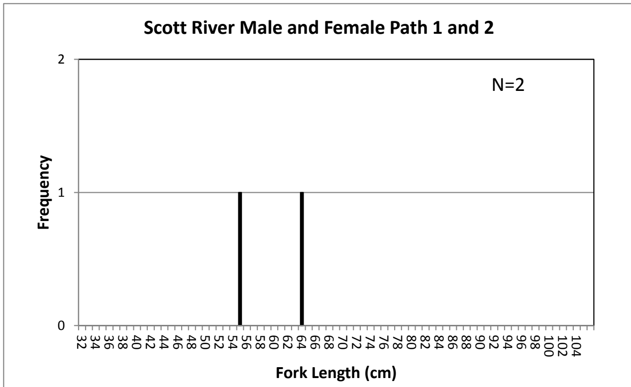
Figure 11. Length frequency distribution of Female and Male Coho Salmon observed (N=2) during the cooperative spawning ground survey (1) and the SRCD (Voight 2021) spawning ground survey (1) in the Scott River 2021-2022.
