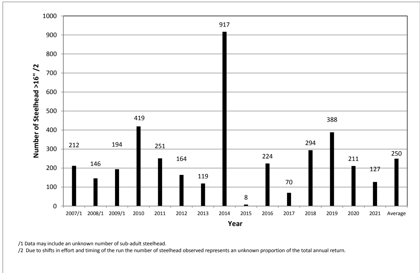
Figure 22. Number of observed steelhead >16" at the Scott River Fish Counting Facility from 2007 to 2021.
