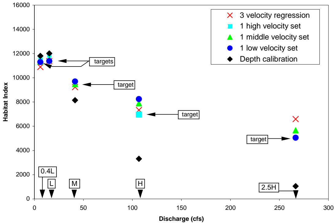
Figure 3. Example of habitat index predictions for five velocity simulation methods over a range of flows (top) and five target flow levels consisting of each calibration flow and 40% of low and 250% of high calibration flow (bottom) for shallow/slow habitat suitability criteria.
