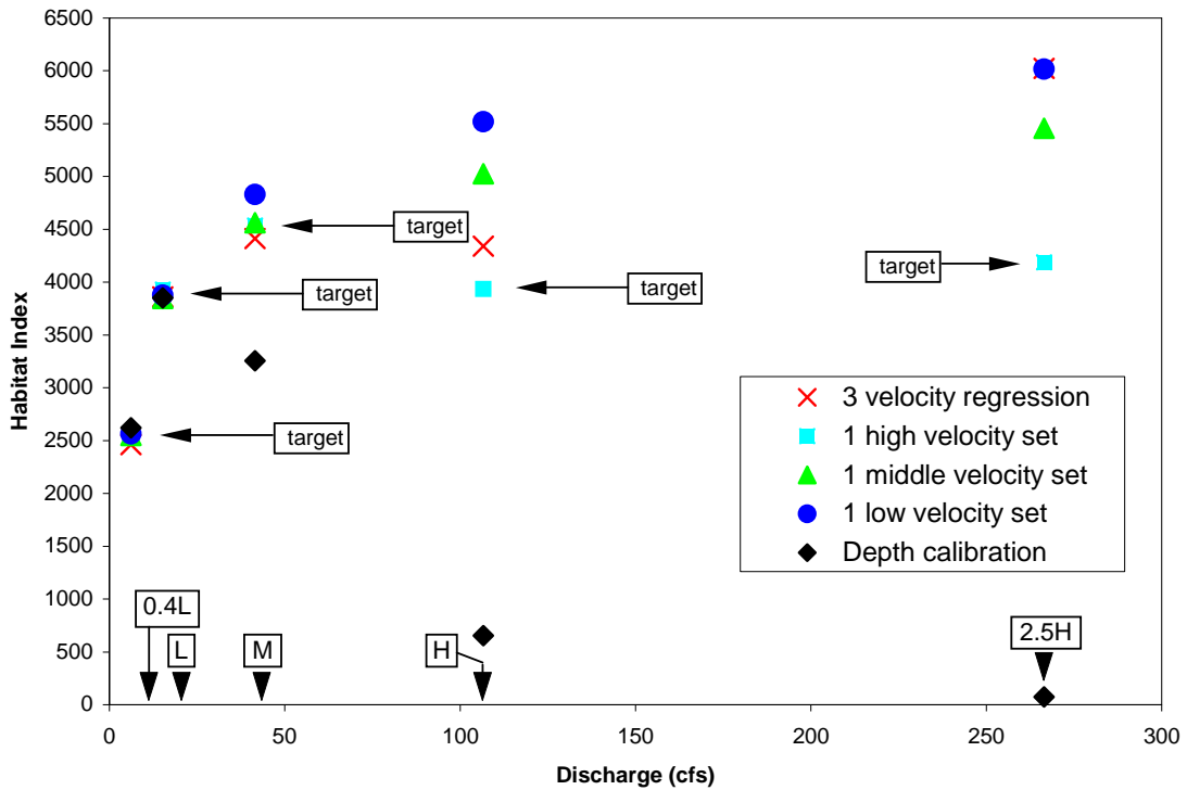
Figure 1. Example of habitat index predictions for five velocity simulation methods over a range of flows (top) and five target flow levels consisting of each calibration flow and 40% of low and 250% of high calibration flow (bottom) for deep/slow habitat suitability criteria.
