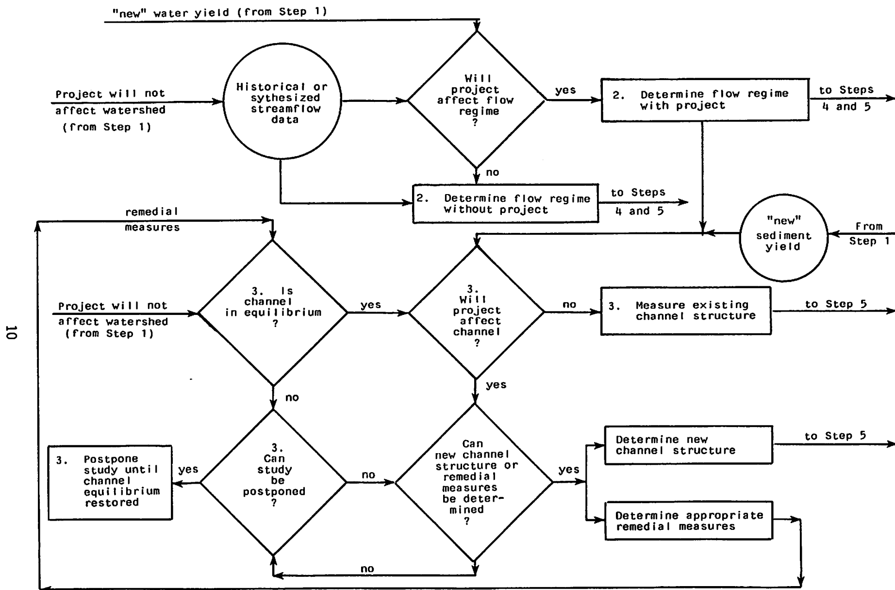
Figure 3. Step 2 (top): Determine flow regime with and without project; and Step 3 (bottom): Determine channel structure with and without project.
