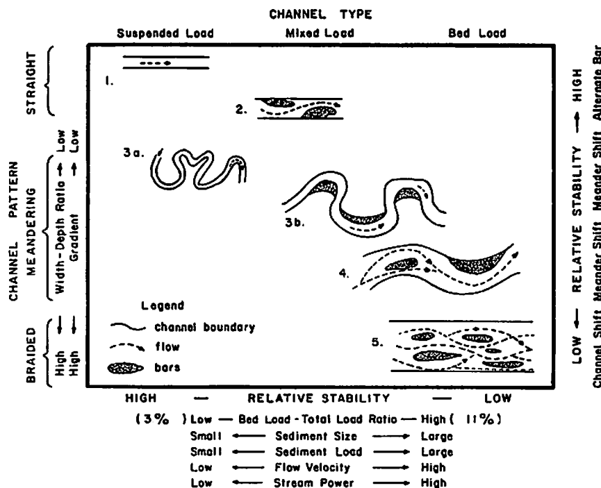
Figure 35. Classification and stability of alluvial channels (from Shen et al. 1981).
