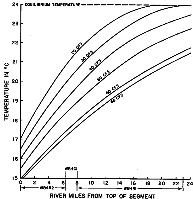
Figure 13. Example of temperature profile overlaid on a segment having multiple study sites (from Figure 12).
